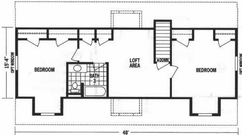
PROPOSED UNFINISHED SECOND FLOOR (AVAILABLE WITH 12/12 ROOF ONLY)
